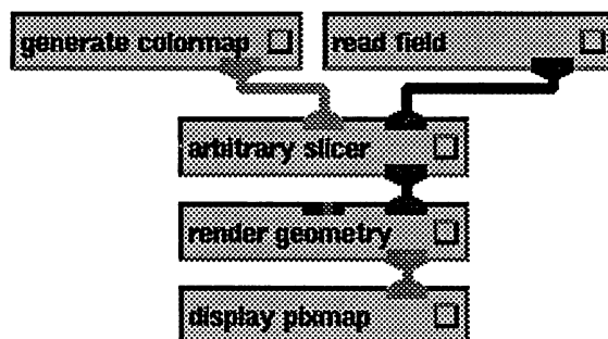
Figure 1-11. One-Mapper Geometry Network
