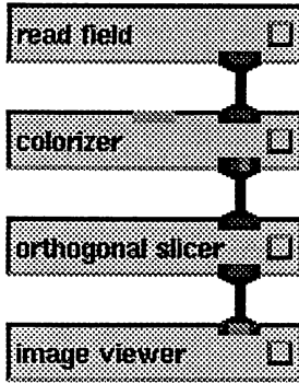
Figure 1-15. Simple Imaging Technique Network
