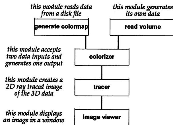
Figure 1-2. Simple Network of AVS Modules
