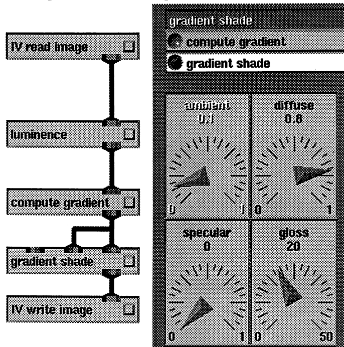
Figure 4-18. Network and Control Panel for Gradient Shade Technique
