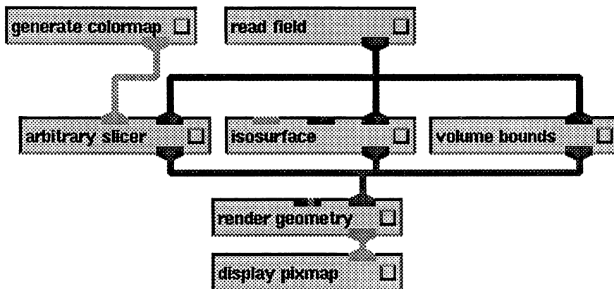
Figure 1-13. Three Geometry Mapper Modules in Parallel
