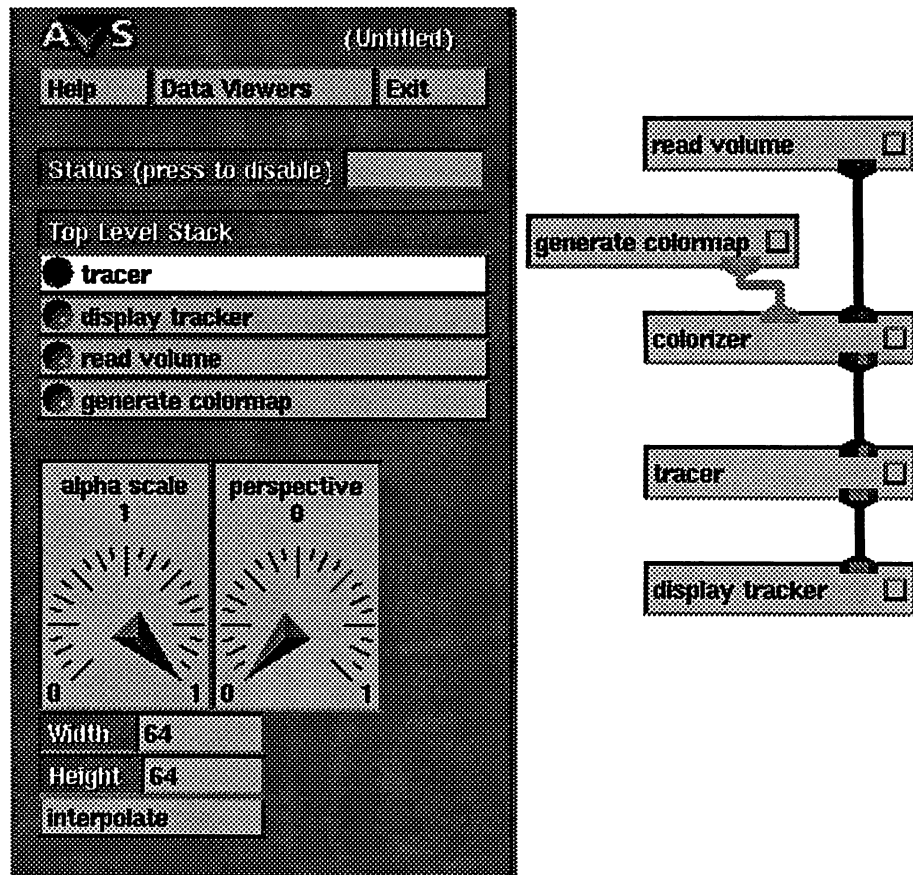
Figure 1-4. A Module's Interface: Control Panel
