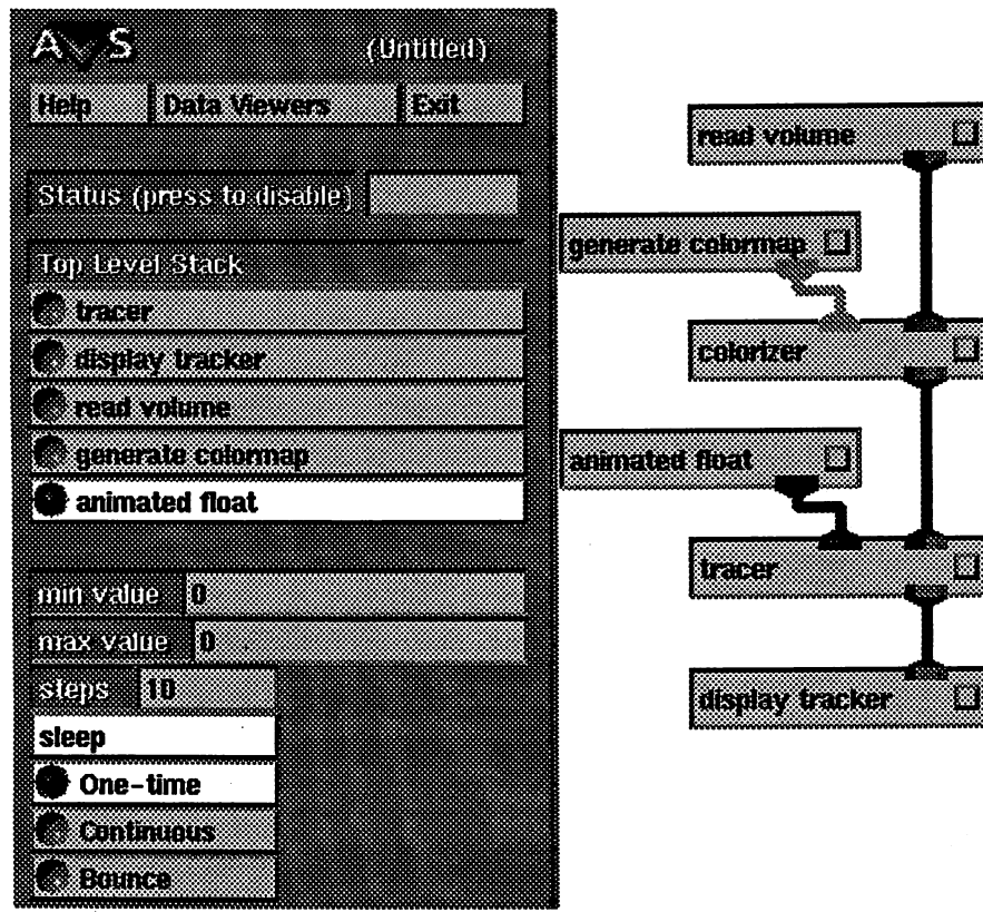
Figure 6-18. Organization of the Network Control Panel
