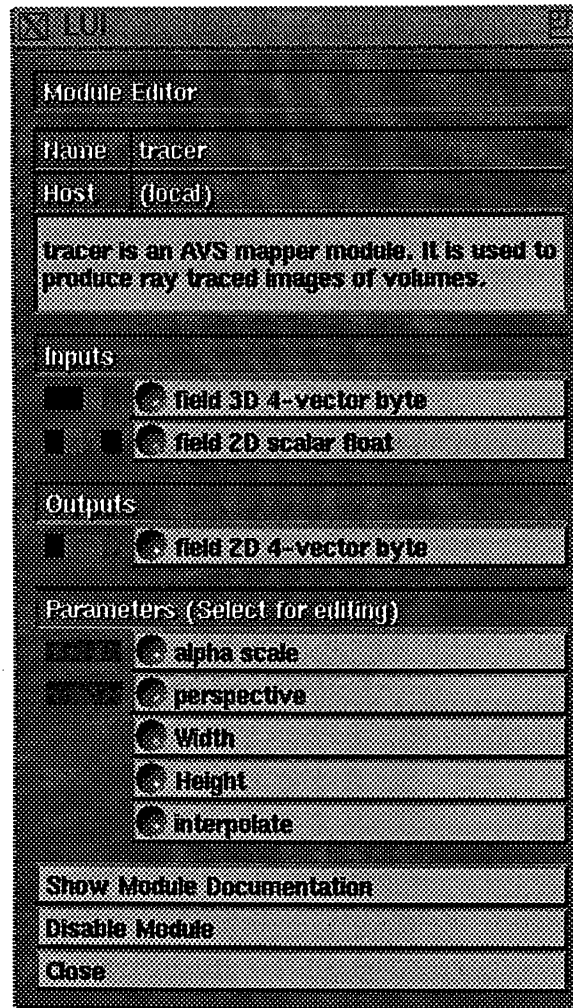
Figure 6-5. The Module Editor
