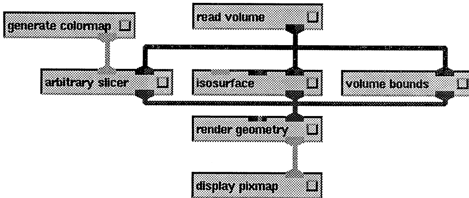
Figure 5-3. A Network that Produces Three Geometries
