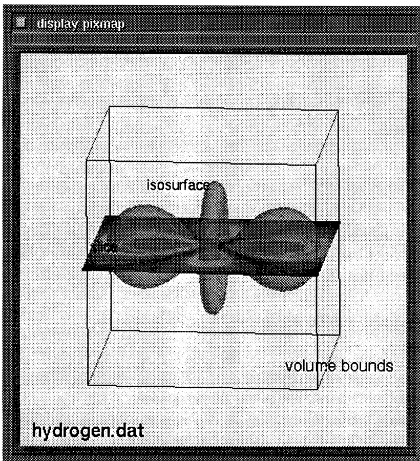
Figure 5-34. Scene with Three Labels and a Title
