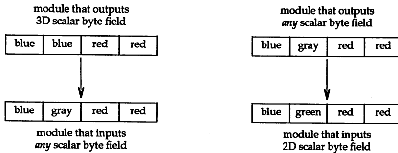
Figure 6-13. Gray Color-Coding as Wildcard Value
