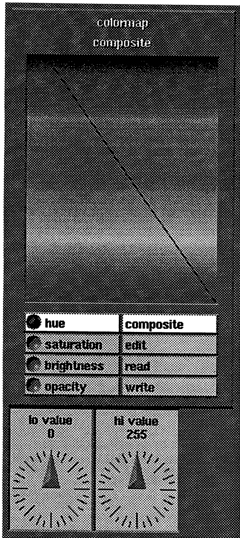
Figure 6-30. Colormap Editor Widget
