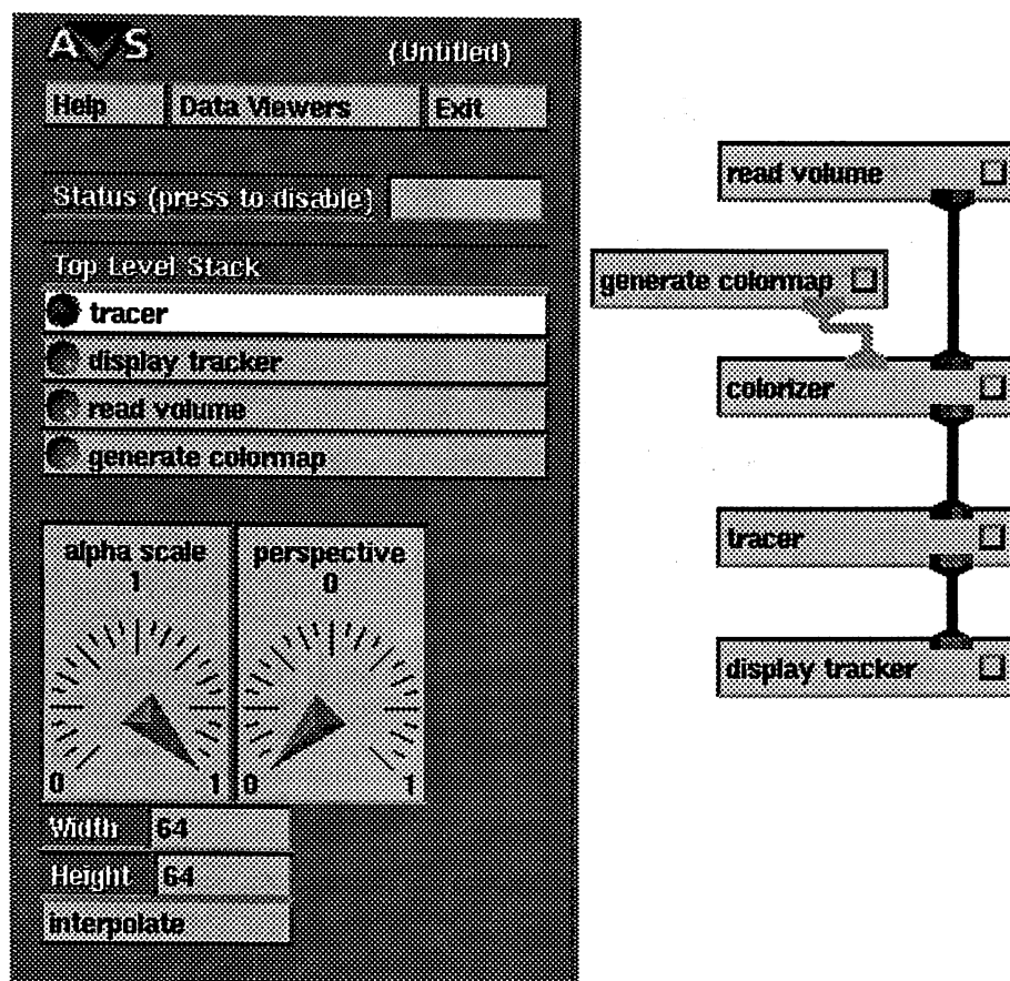
Figure 6-7. Network Editor Control Panel and Network
