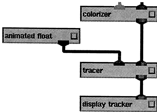
Figure 6-15. Animated Float Parameter Module Connected to Tracer
