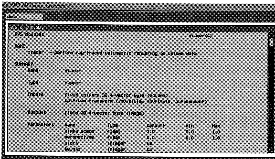
Figure 6-10. Module Help Browser
