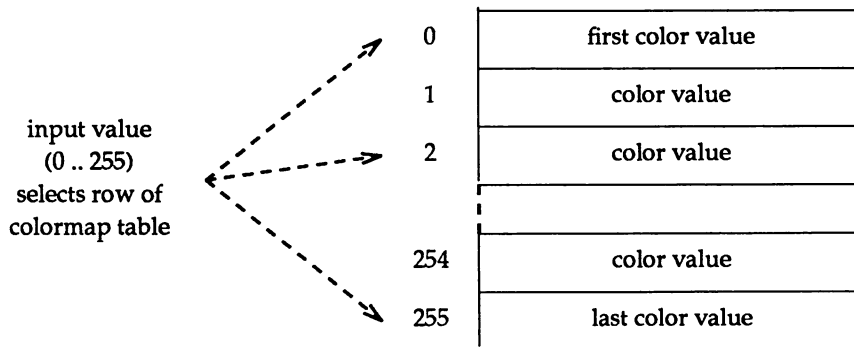
Figure 1-1. AVS Colormap Lookup
