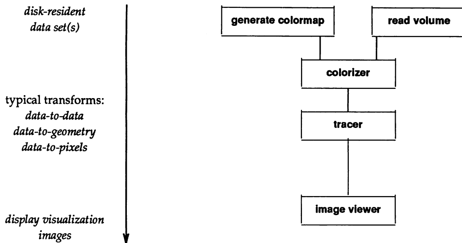
Figure 1-9. Data Flow in a Network
