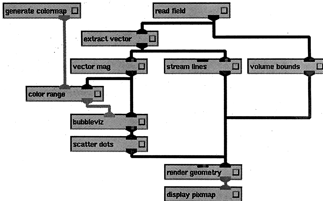
Figure 1-24. A Network to Visualize Vectors
