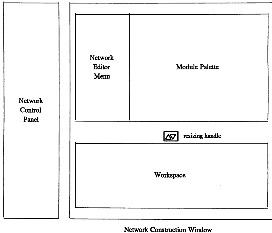
Figure 6-1. Network Control Panel and Network Construction Window
