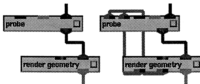
Figure 6-9. Upstream Data Ports Made Visible
