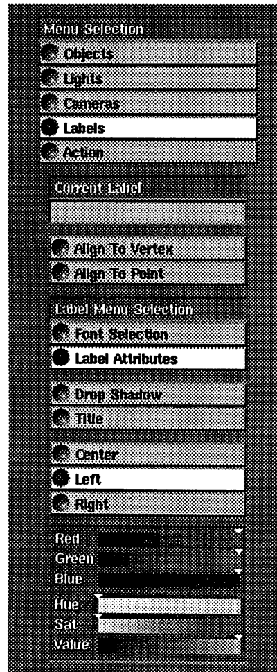
Figure 5-33. Labels Menu Selections
