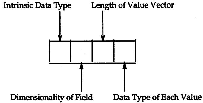
Figure 6-12. Color-Coding for Field Input/Output Ports
