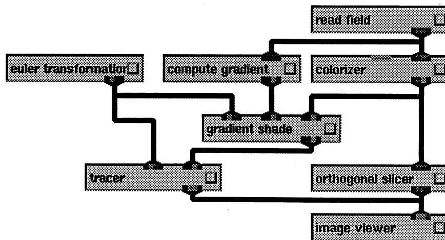
Figure 1-17. Tracing, Gradient Shading, and Slicing Combined
