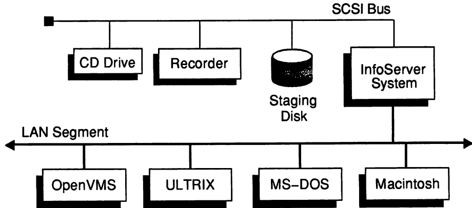
Figure 4-1 Recording Configuration
