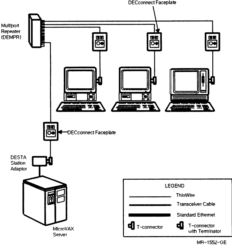
Figure 4-1 Basic DECconnect Faceplate Configuration
