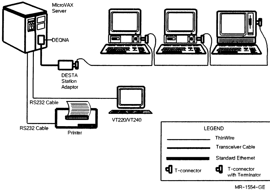
Figure 4-3 Daisy-Chain Configuration
