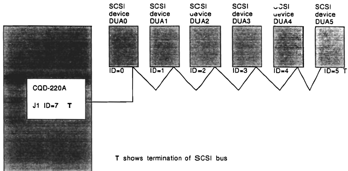
Figure 3-7: SCSI ID and Cabling
