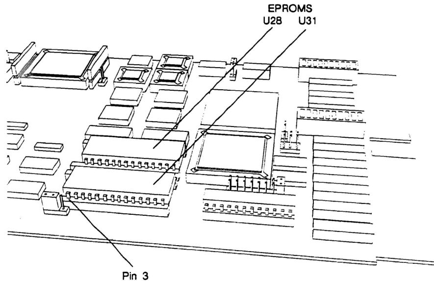
Figure 3-4: Eprom setting
