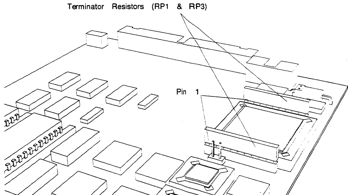
Figure 3-3: Terminator Resistor Location
