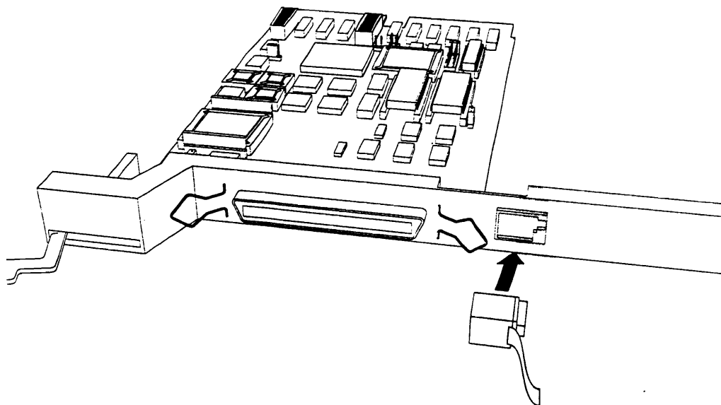
Figure 4-2: CQD-223A RS-232 Port
