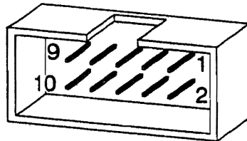
Figure C-1: Pin Locations for J2 (CQD-220A) and J3
