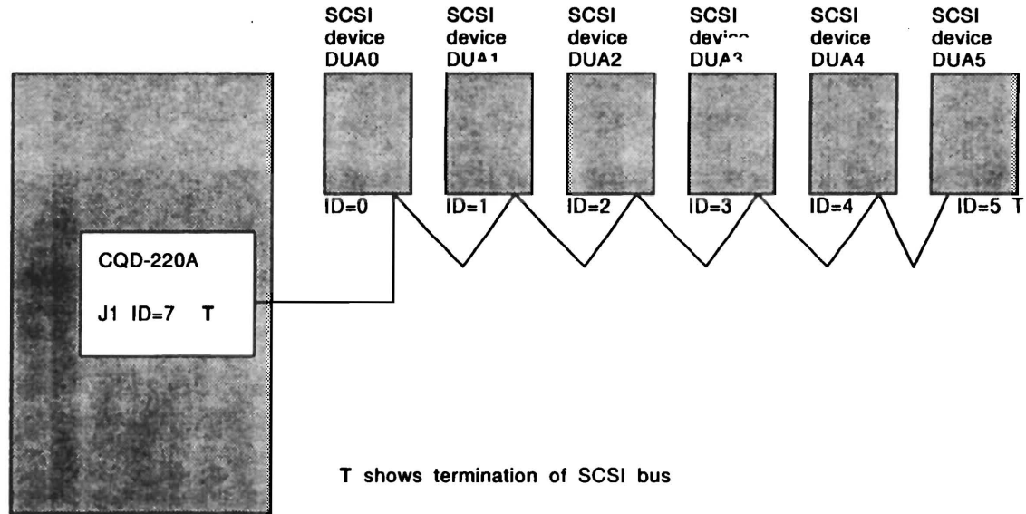
Figure 1: SCSI ID and Cabling
