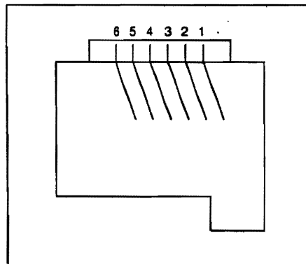
Figure C-2: Pin Locations for J2B (CQD-223A)
