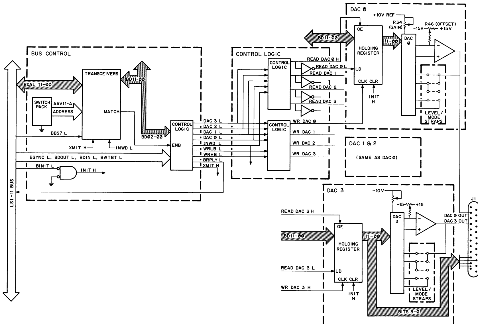
Figure 4-1 AAV11-A Block Diagram
