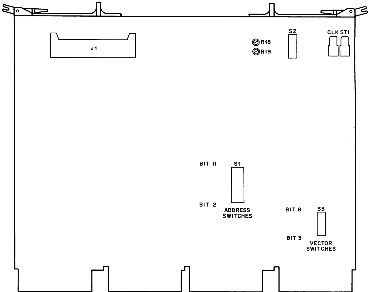
Figure 3-1 KVV11-A Connectors, Switches, and Controls
