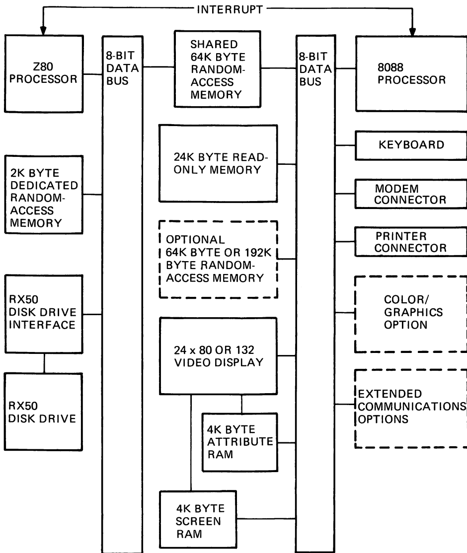
Figure 1-2. Rainbow 100 Computer, Block Diagram
