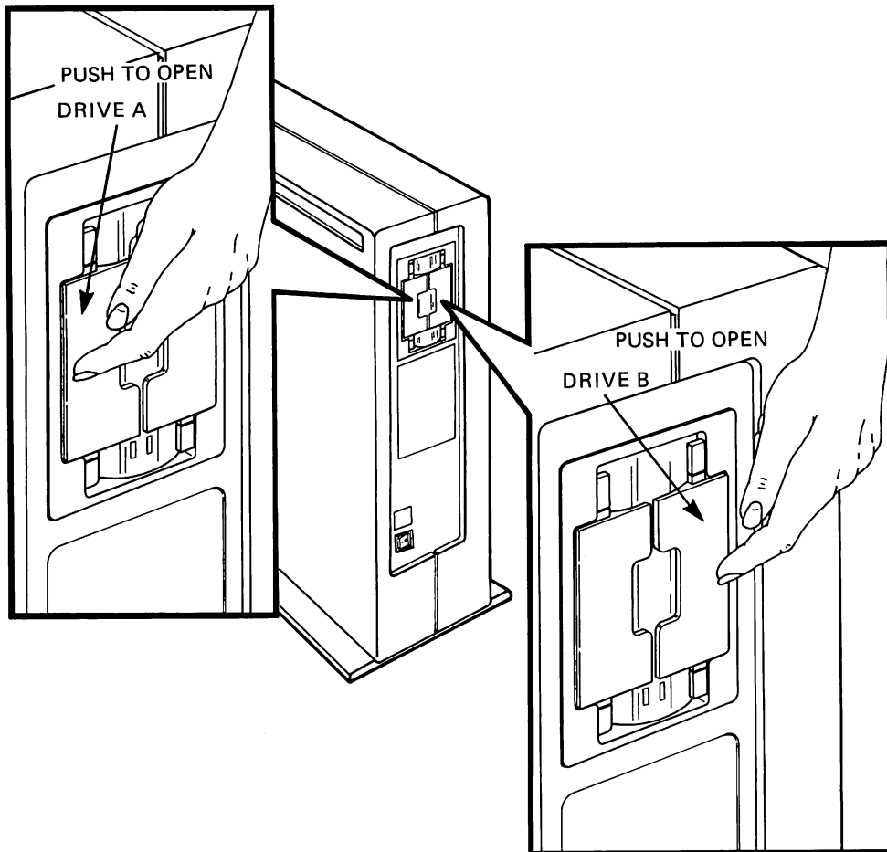
Figure 5-5. Opening the Disk Drive Doors When Using the Floor Stand
