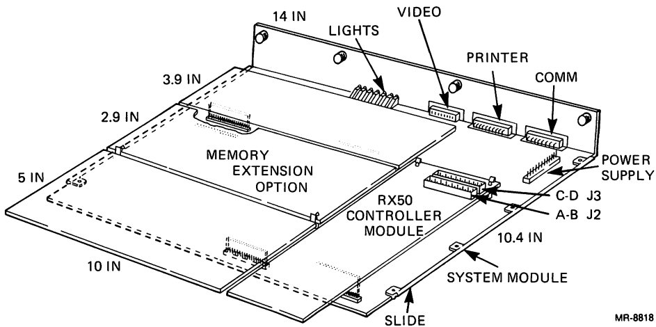
Figure 1-6. System Module
