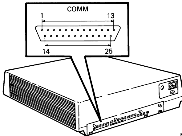
Figure 4-4. Communications Connector Pin Numbers
