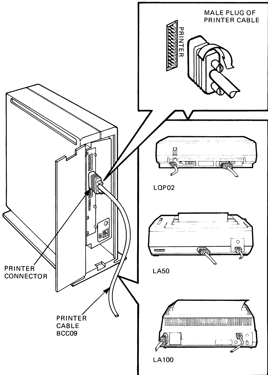
Figure 3-4. Connecting a Printer to the System Unit in the Floor Stand
