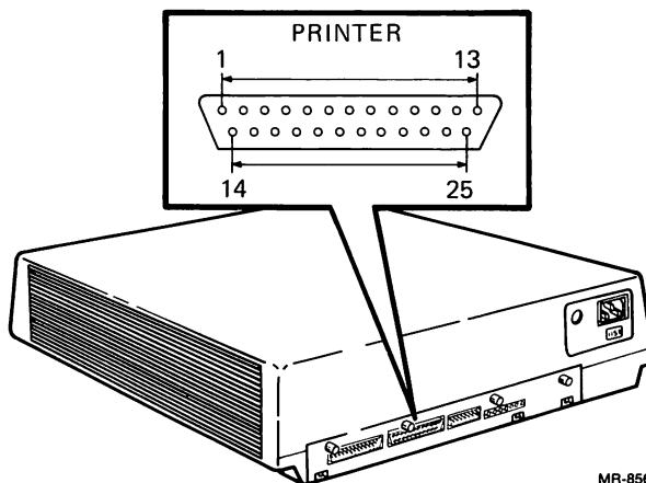
Figure 3-2. Printer Connector on the System Unit
