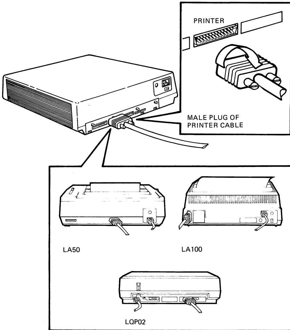
Figure 3-3. Connecting a Printer to the System Unit (without Floor Stand)
