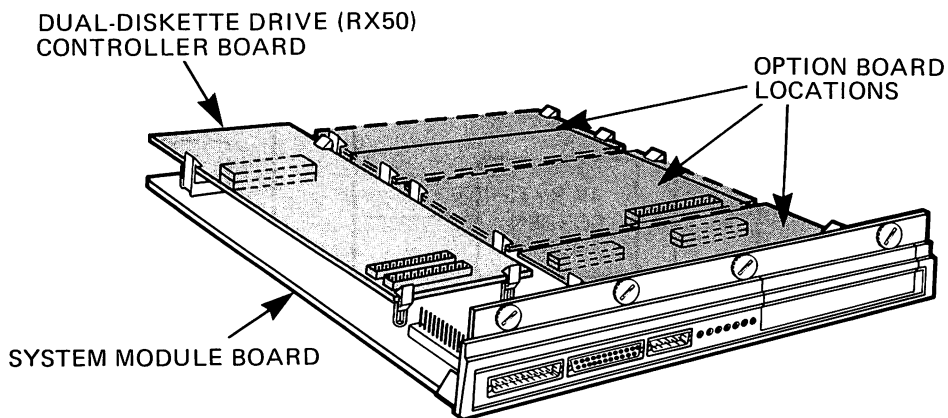
Figure 1-8. System Module
