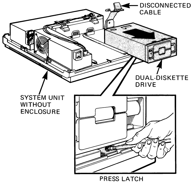
Figure 1-5. Removal of Dual-Diskette Drive
