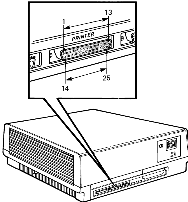
Figure 4-2. Printer Connector on the System Unit
