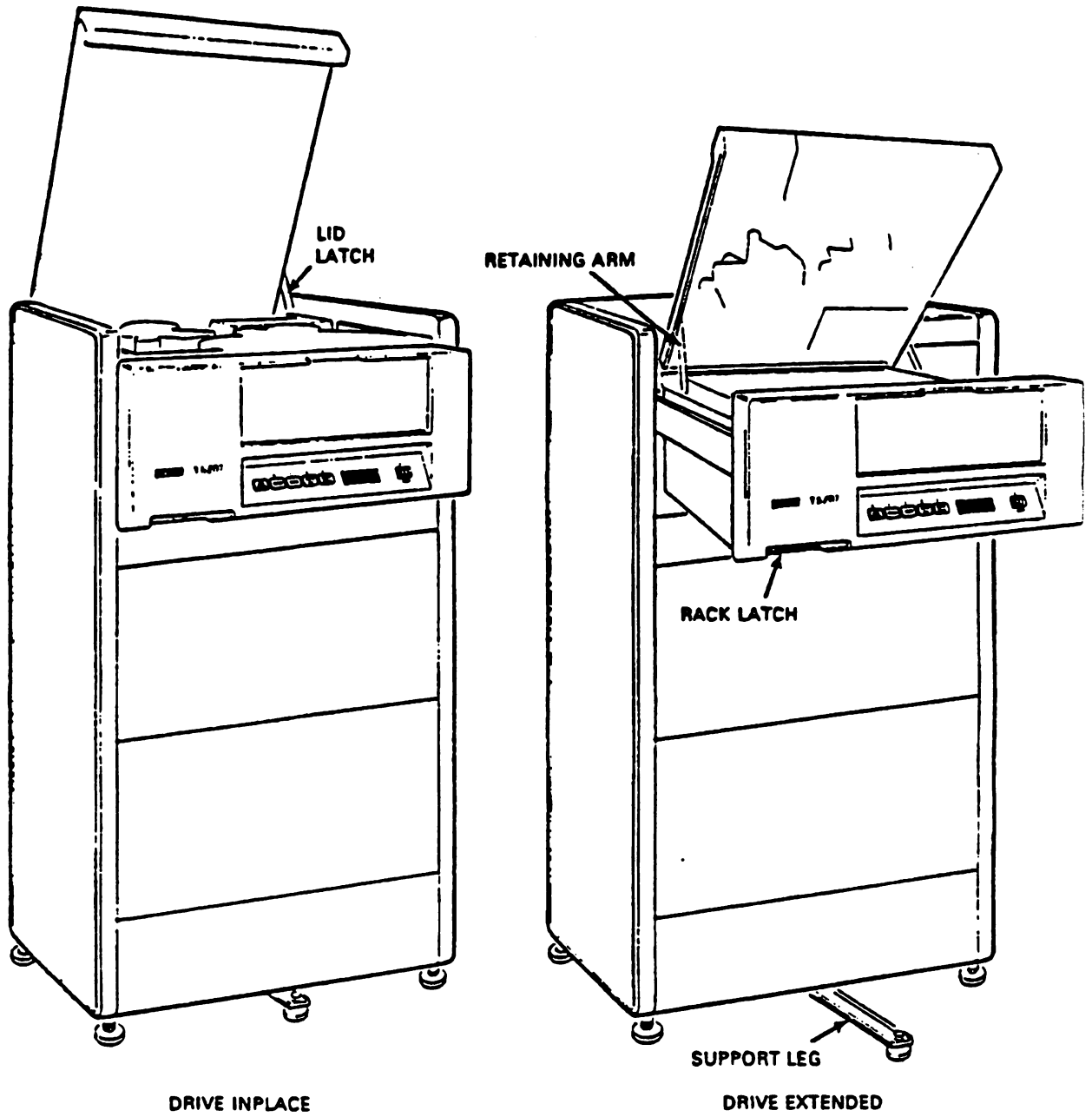
Figure 2-14: Opening Cabinet Lid
