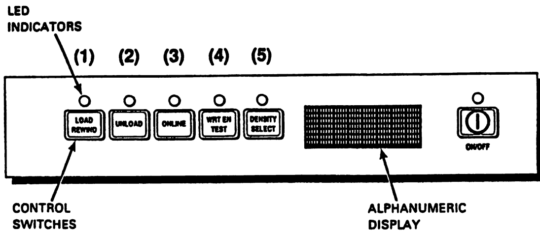
Figure 3-1: Front Panel
