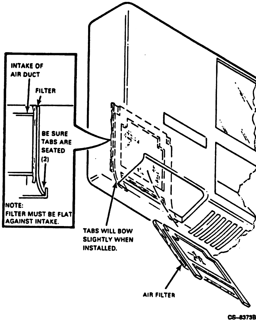
Figure 4-2: Air Filter
