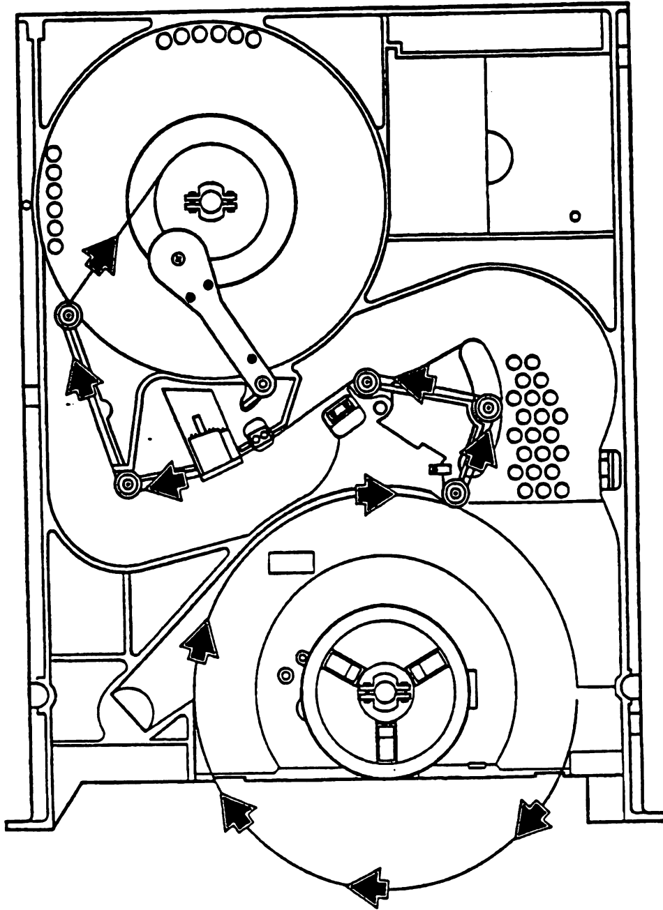
Figure 3-5: Tape Path
