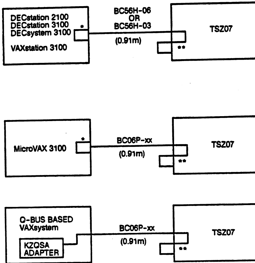
Figure 2-5: Typical Standalone SCSI Configurations
