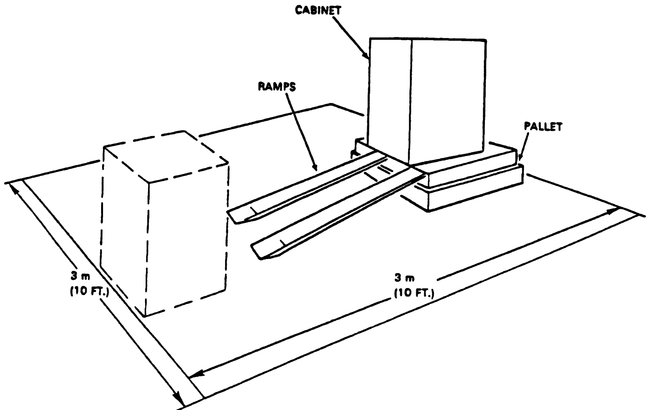
Figure 2-8: Cabinet Working Space
