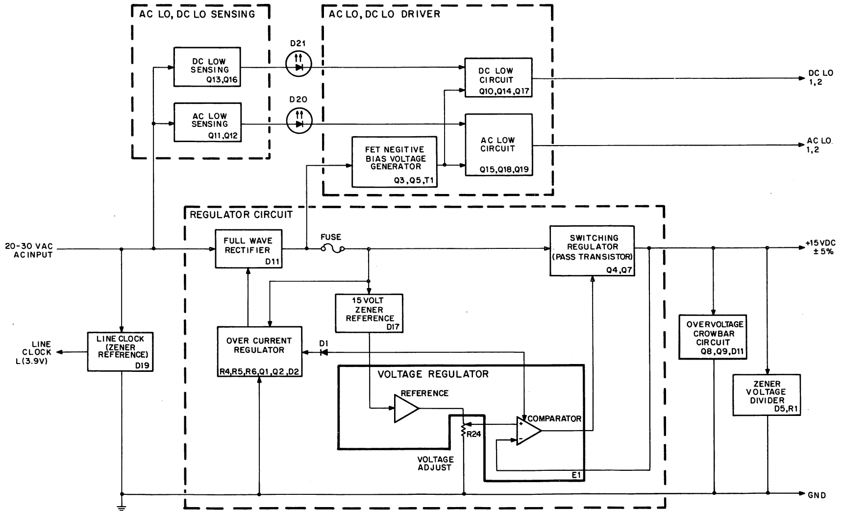
Figure 3-6 5411086 Block Diagram
