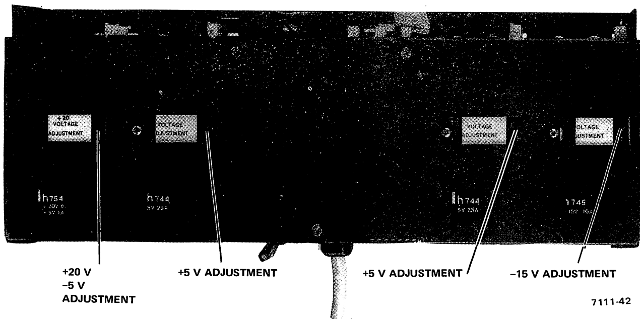
Figure 4-2 Regulator Adjustments
