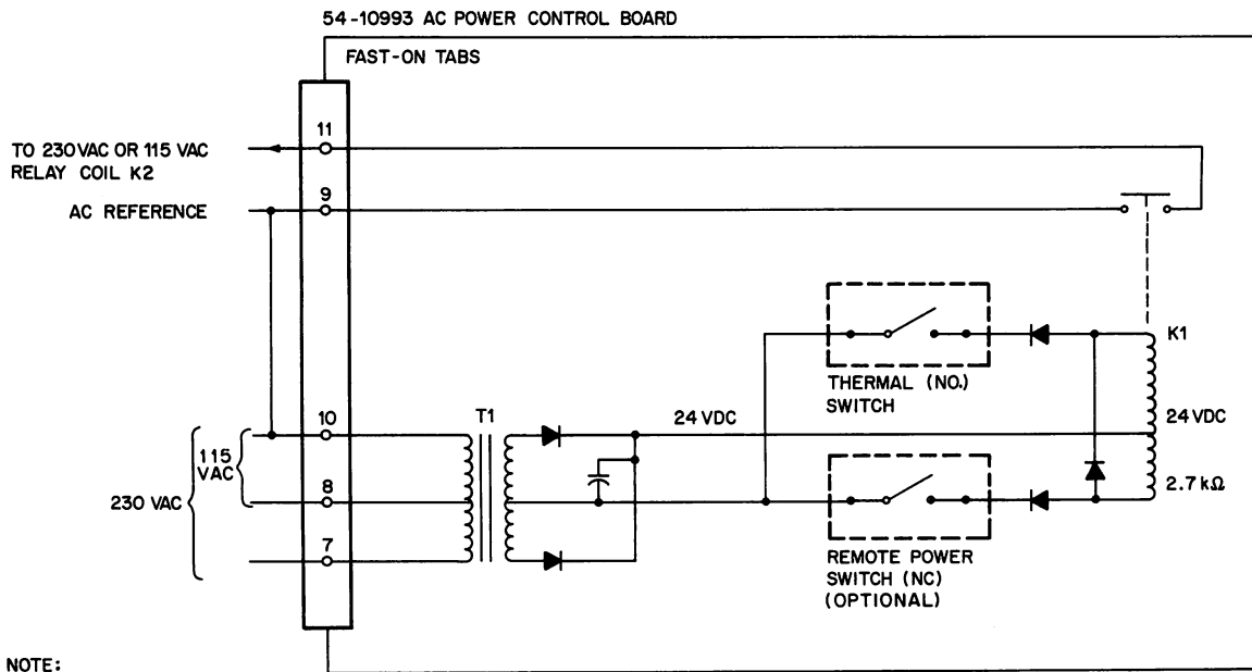
Figure 3-4 230 V Power Configuration
