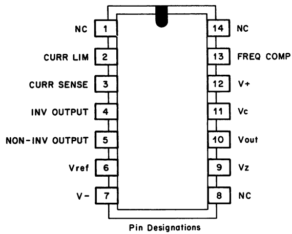
Figure 3-9 Voltage Regulator E1, Simplified Diagram
