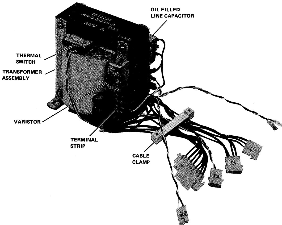
Figure 4-8 Transformer Assembly
