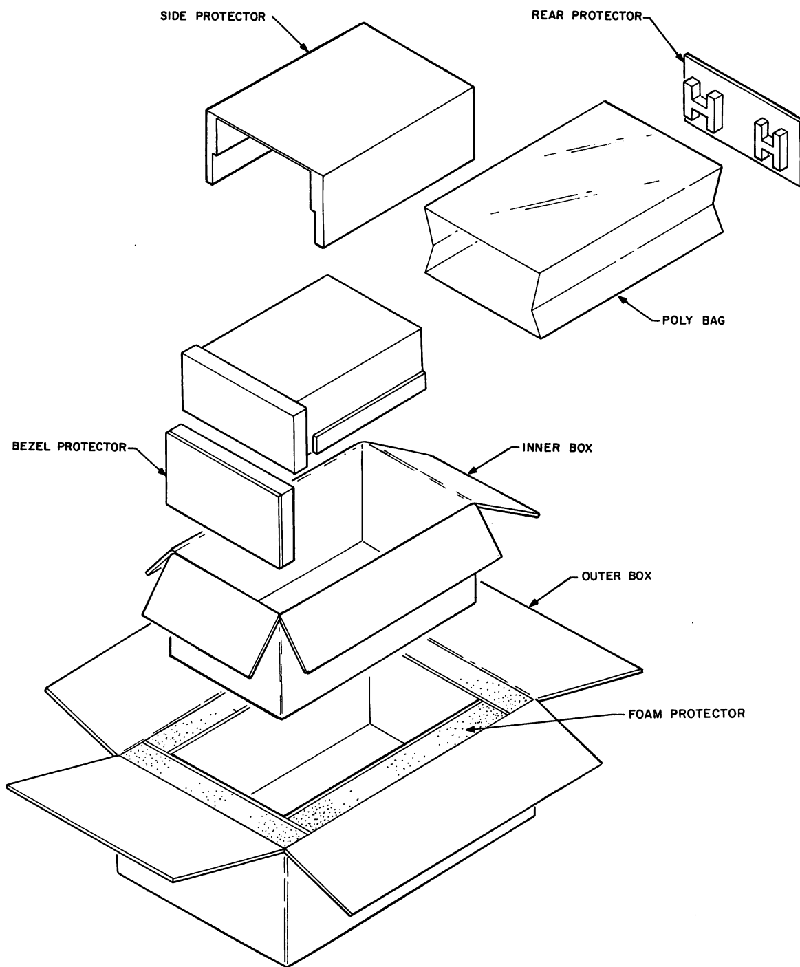
Figure 5-1 BA11-K Packaging
