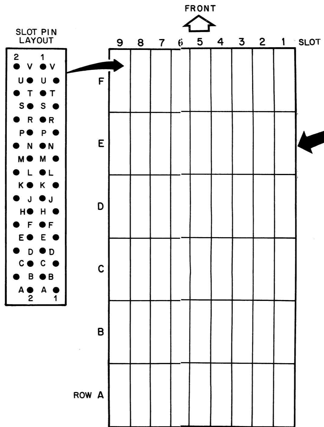
VIEW FROM WIRE WRAP PIN SIDE. COMPUTER IN MAINTENANCE POSITION
