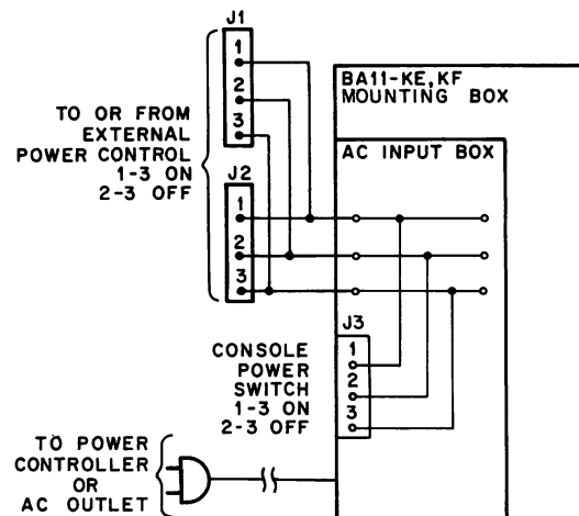
Figure 5-3 Power Control
