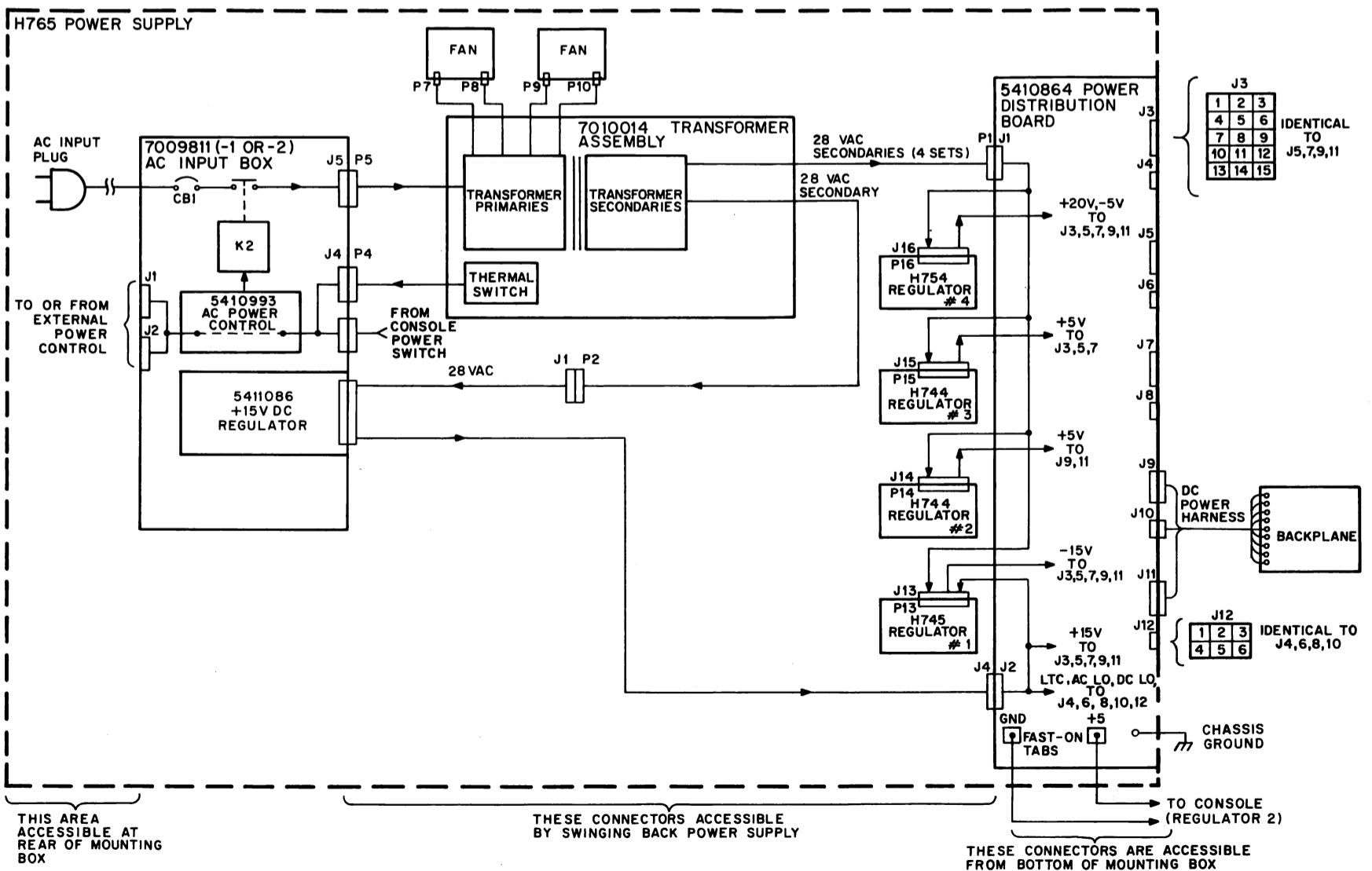
Figure 3-1 Power System Functional Block Diagram
