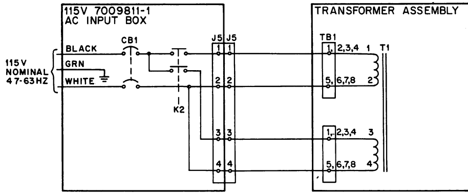
Figure 3-3 115 V Power Configuration
