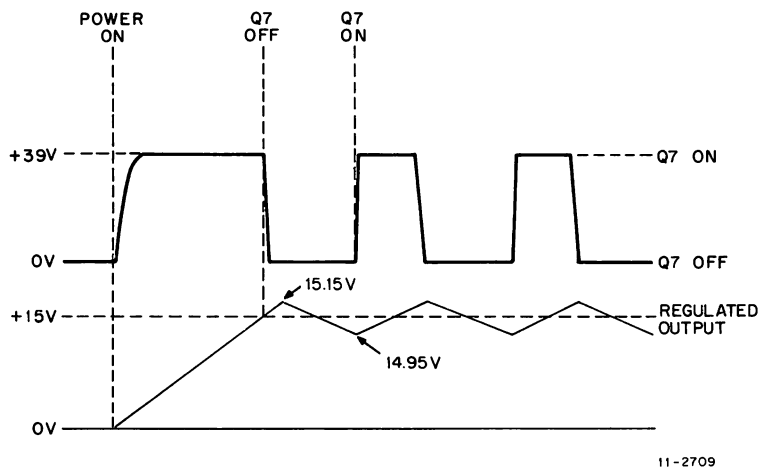
Figure 3-7 5411086 Regulator Waveforms
