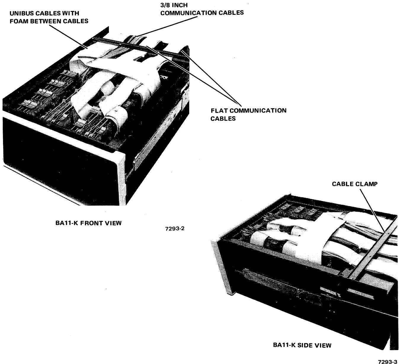
Figure 2-5 Cable Routing
