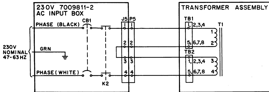
Figure 3-4 230 V Power Configuration
