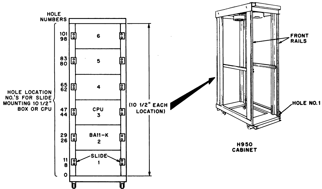
Figure 2-6 BA11-K and CPU Cabinet Mounting Specification
