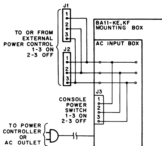
Figure 3-3 Power Control
