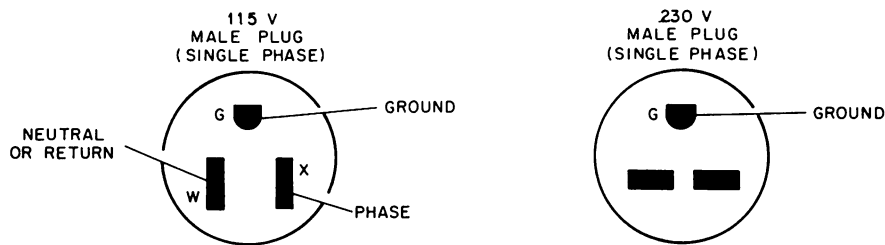
CONNECTOR SPECIFICATIONS
