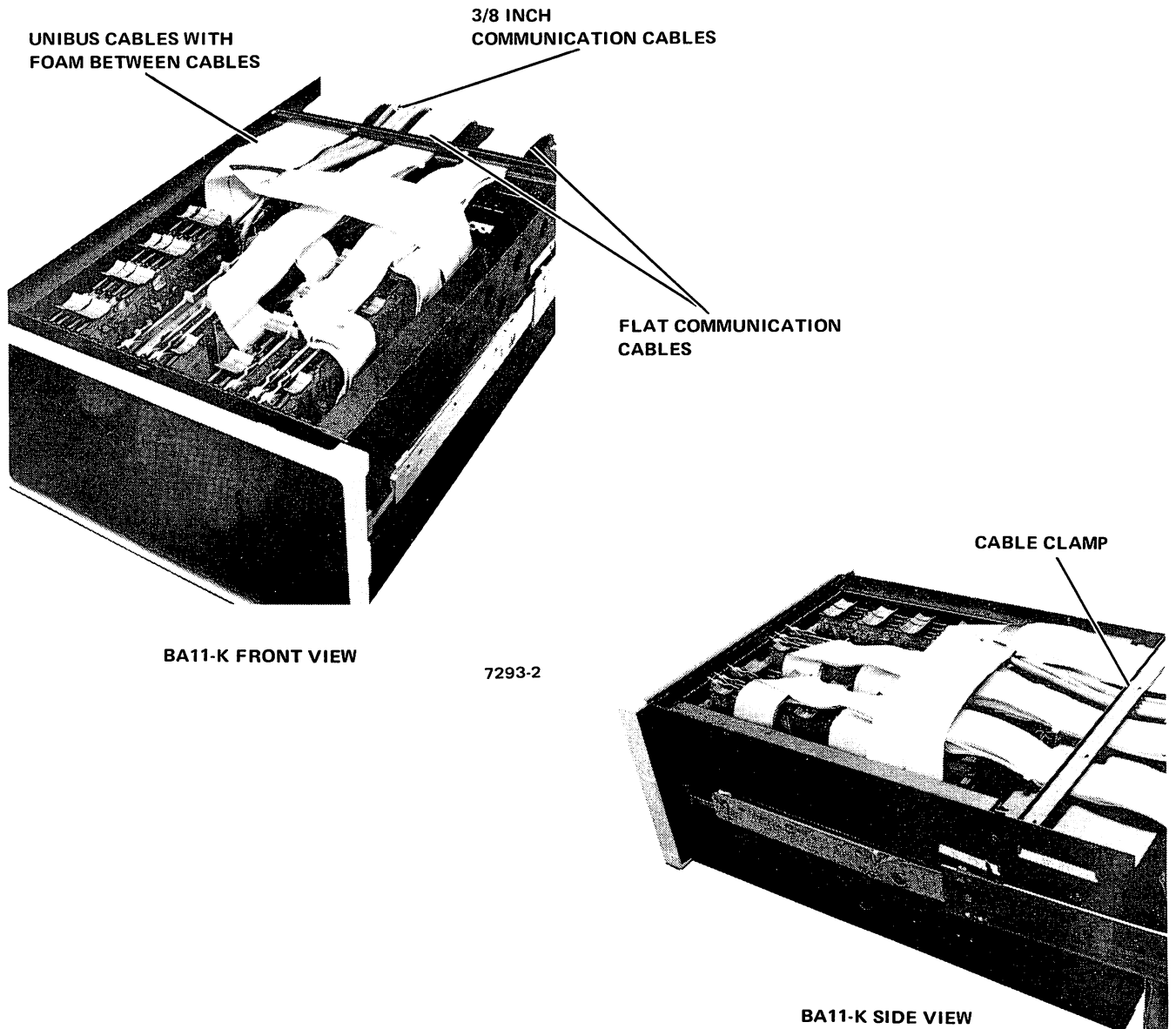
Figure 2-5 Cable Routing
