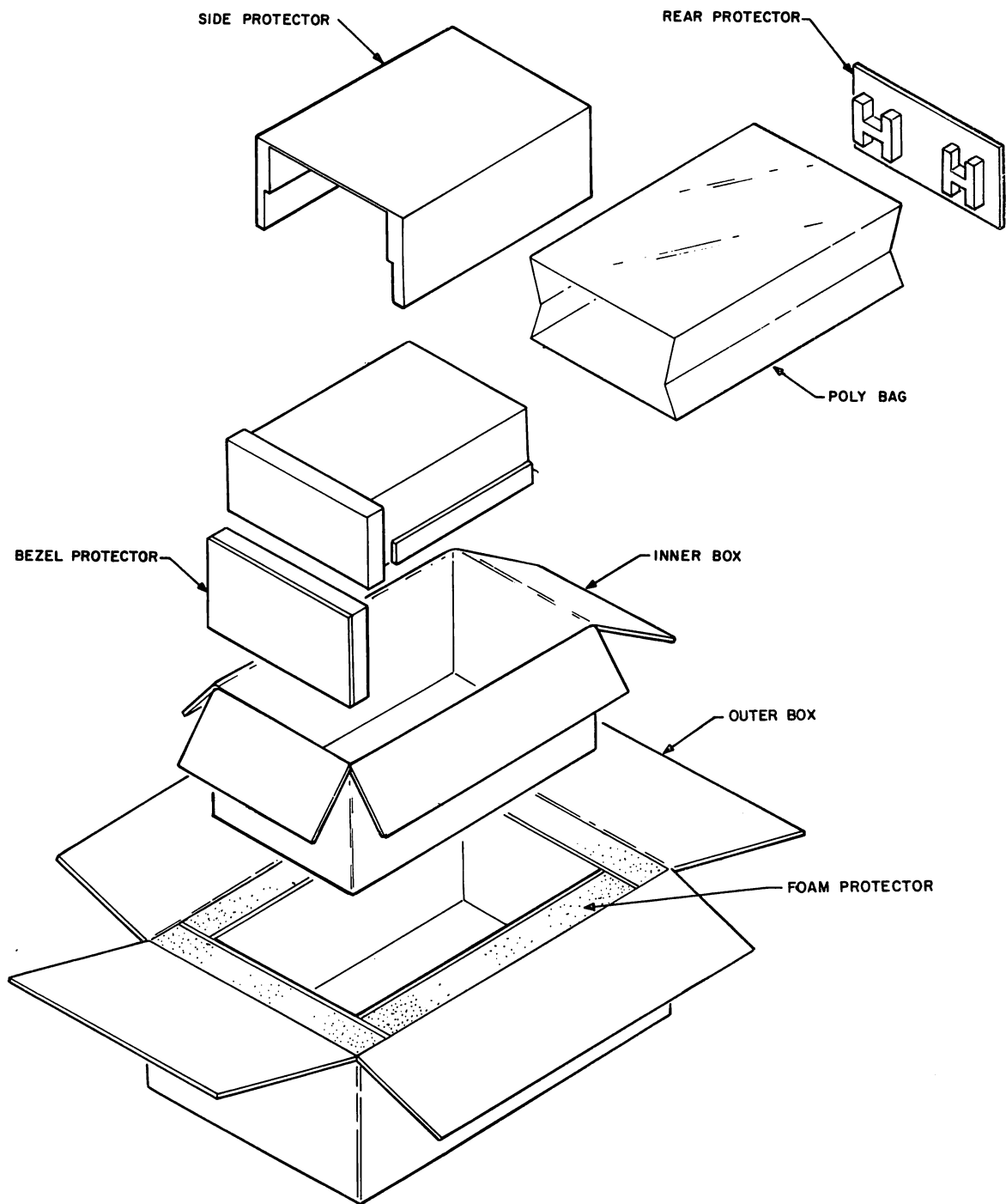
Figure 3-1 BA11-K Packaging
