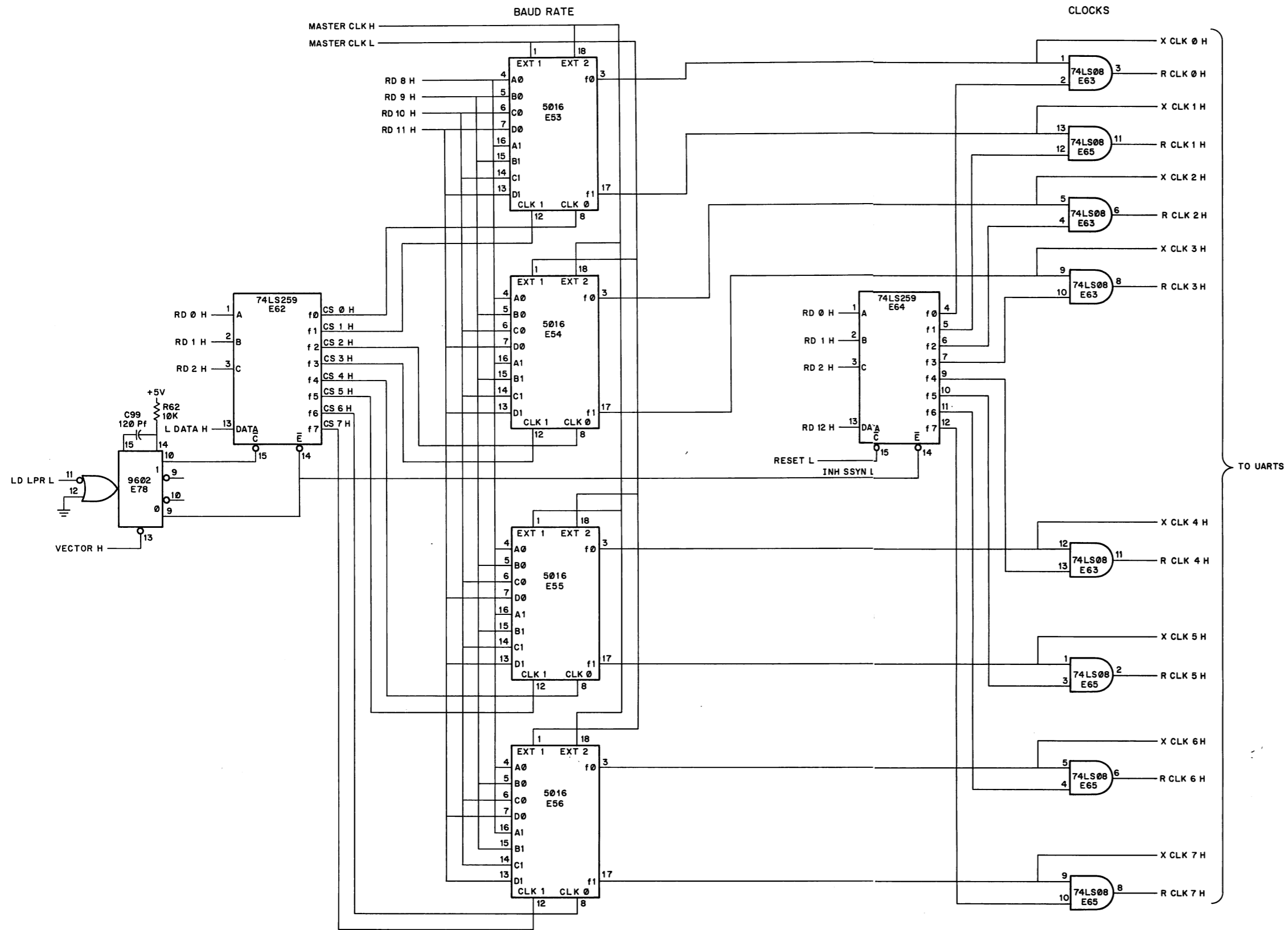
Figure 4-18 LPR Diagram
