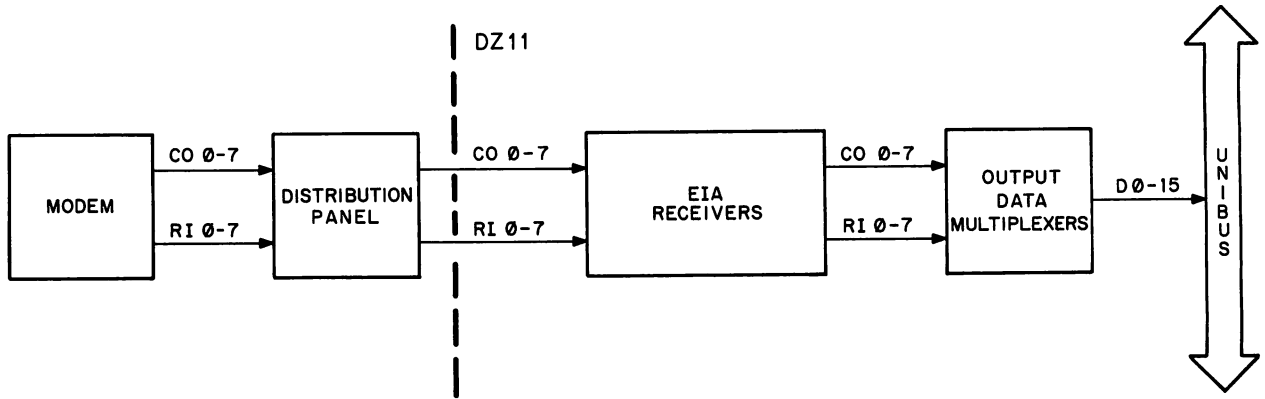
Figure 4-20 MSR Diagram
