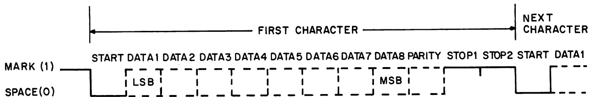
Figure C-1 Format of Typical Input/Output Serial Character
