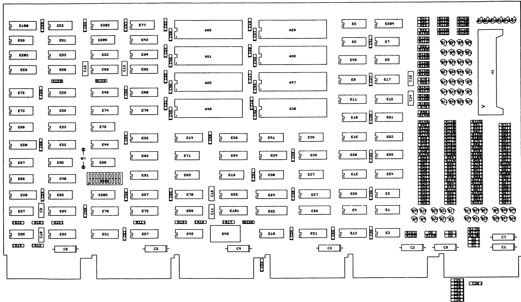
Figure 1-3 DZ11 20 mA Module (M7814)
