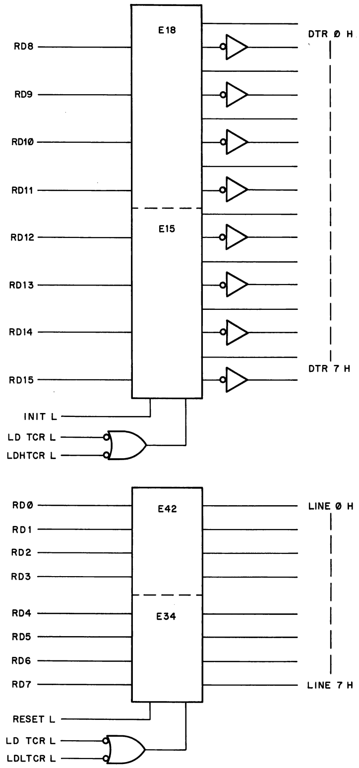
Figure 4-19 TCR Diagram
