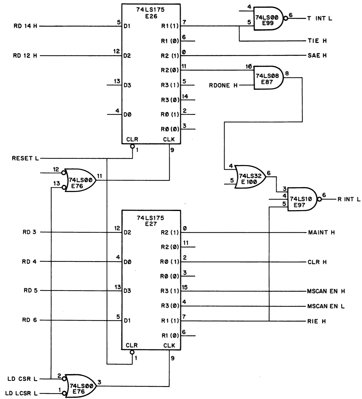
Figure 4-17 CSR Diagram
