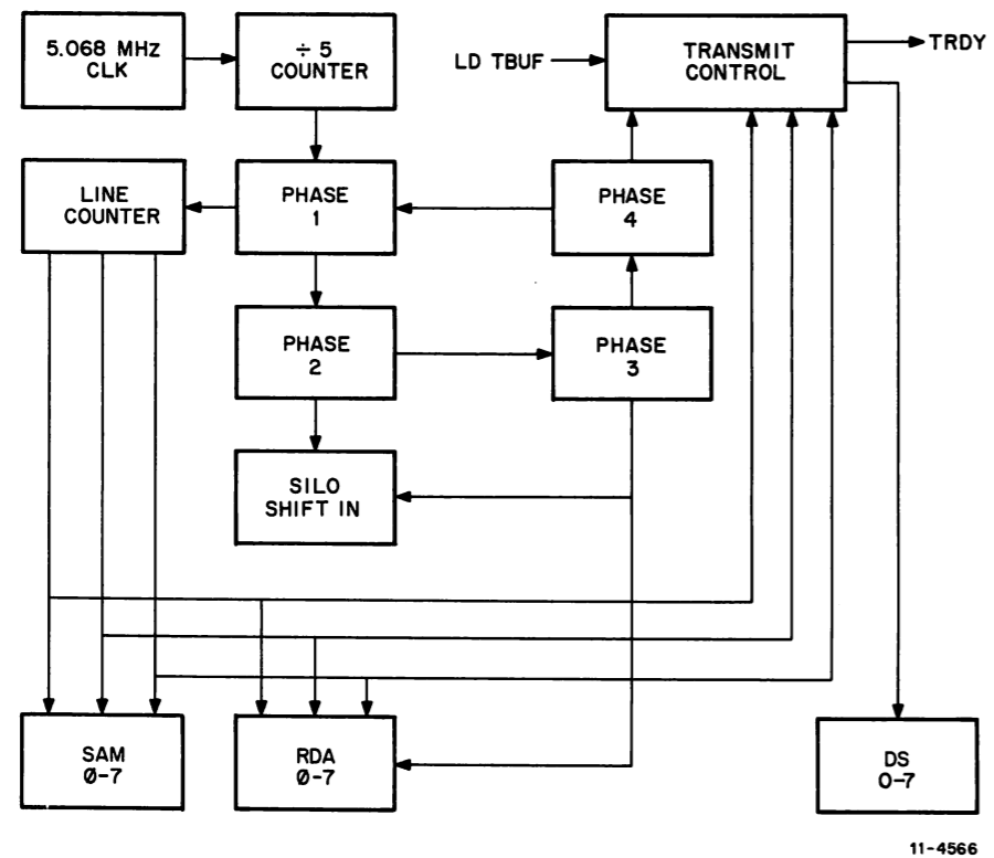
Figure 4-11 Scanner Block Diagram
